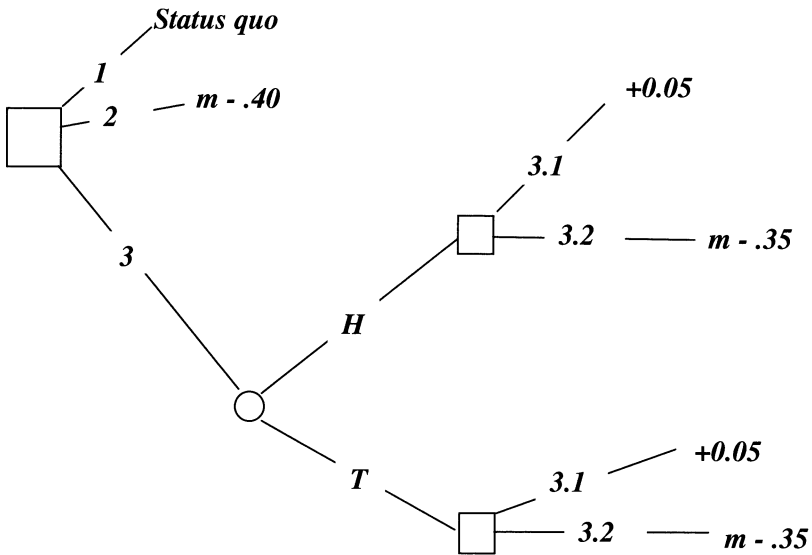
Figure 3: Sequential Decision Problem 2.
