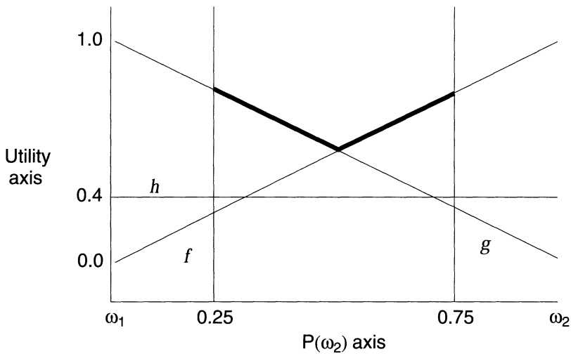
Figure 1: Expected utilities for three acts in Example 15. The thicker line indicates the surface of Bayes solutions.
